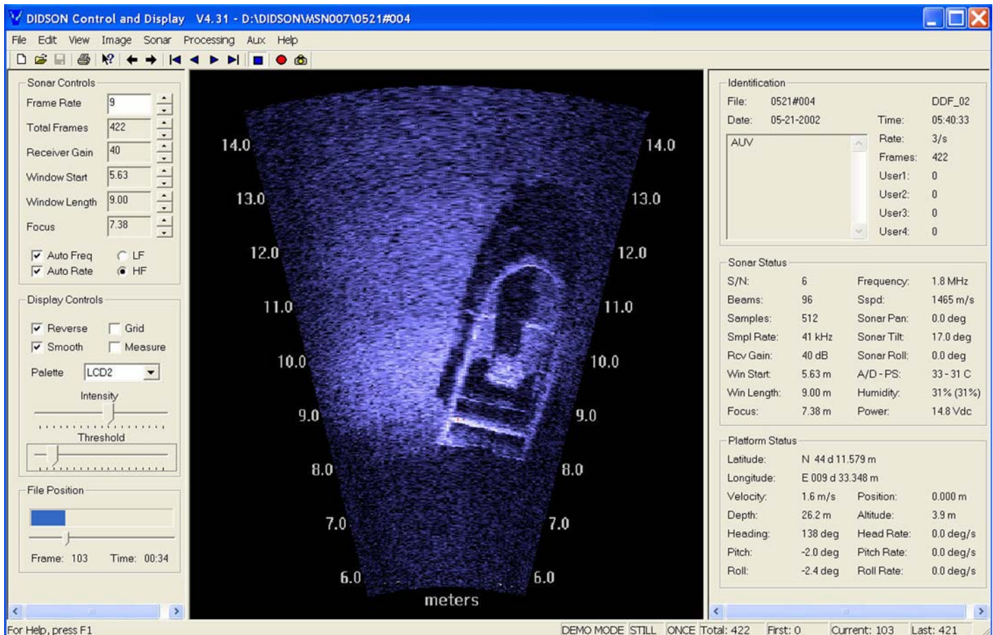
Split-body DIDSON
